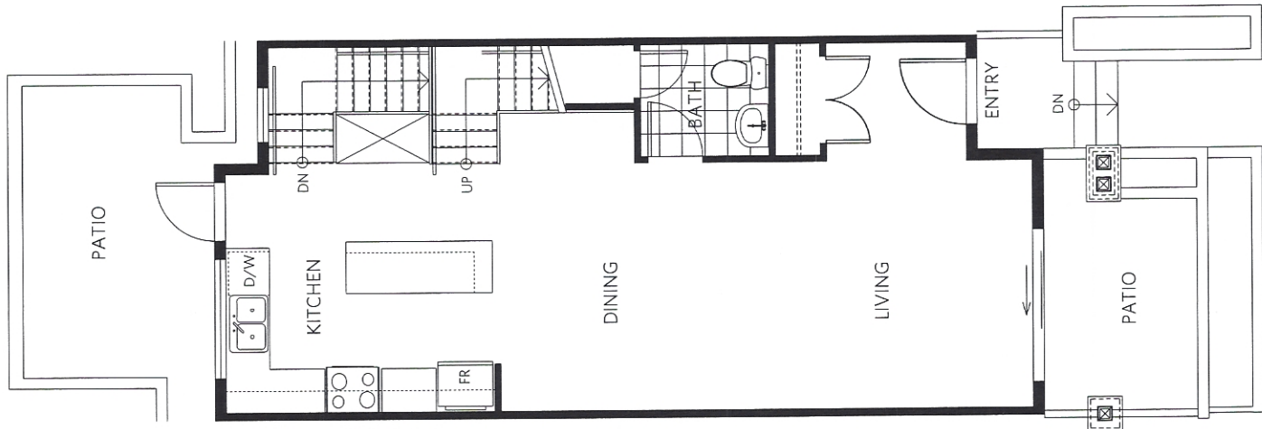
FIRST LEVEL
