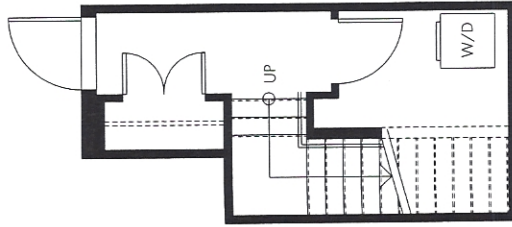
BASEMENT LEVEL
